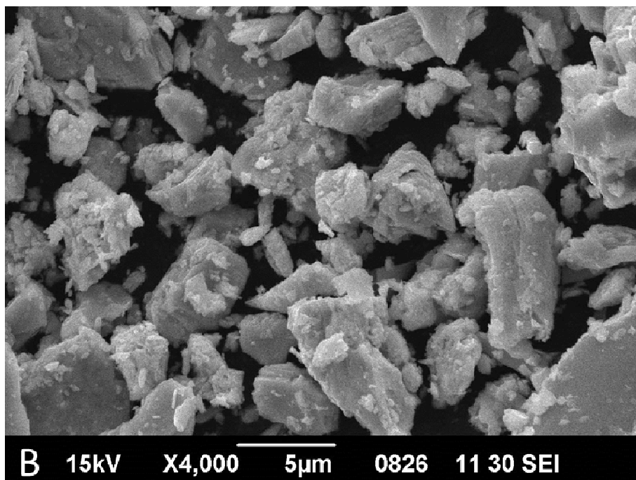
Photo 1. SEM image of our product SnS
